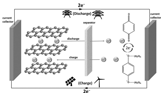
Figure 1. Working principle of the designed liquid battery with \text{H}_2\text{BQ} aqueous solution as catholyte and graphite in aprotic electrolyte as anode. The direction of \text{Li}^+ diffusion inside battery and electron transference in external circuit indicates charge or discharge mode, and curved arrows indicate the direction of the redox reaction in the cathode part. The cartoon on top shows that in discharge mode the battery can provide energy through an electrical grid, and the cartoon below shows sustainable energy sources from wind and sun in charge mode.
